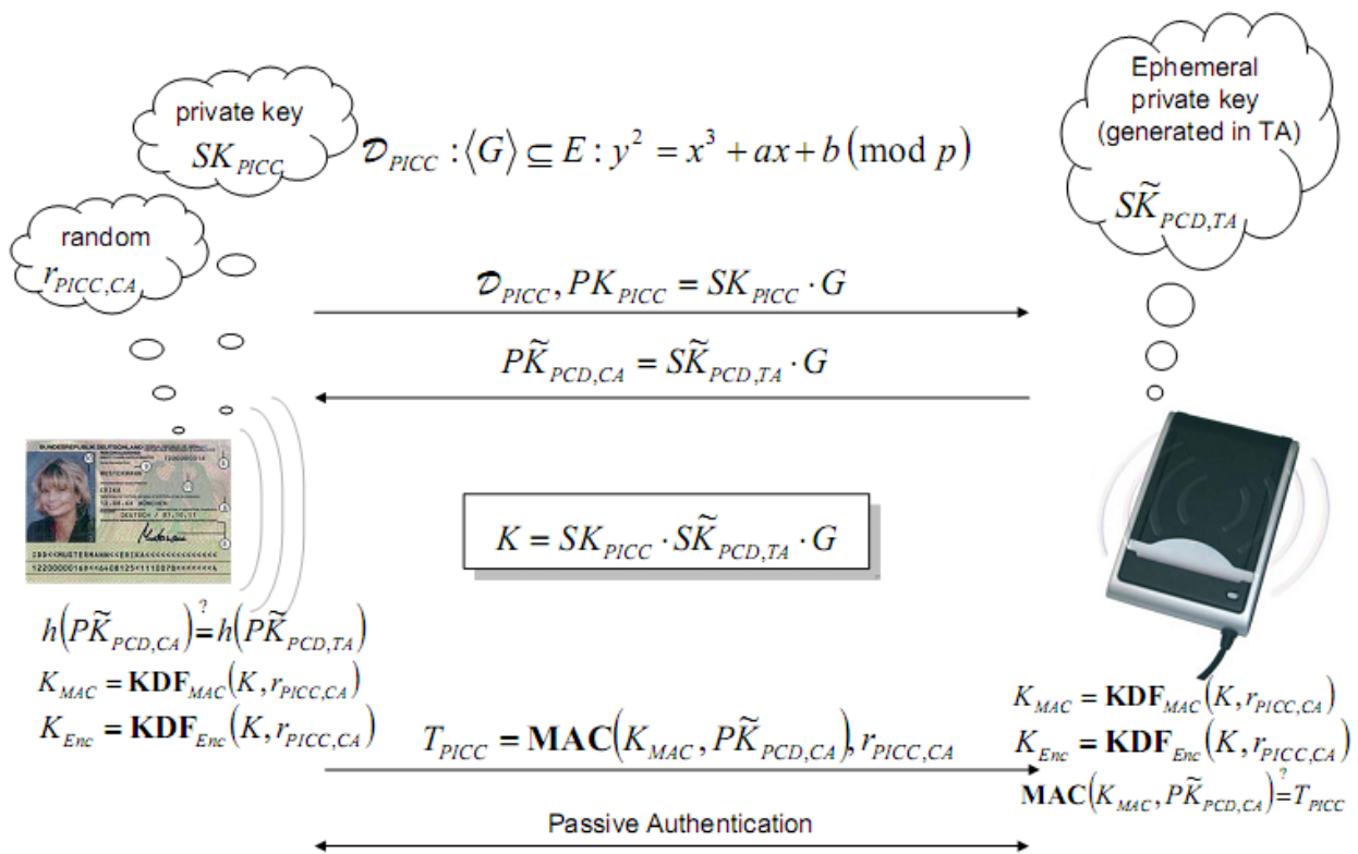
Abbildung 47: Chip Authentication, Version 2 [BSI-TR-03112-7]
