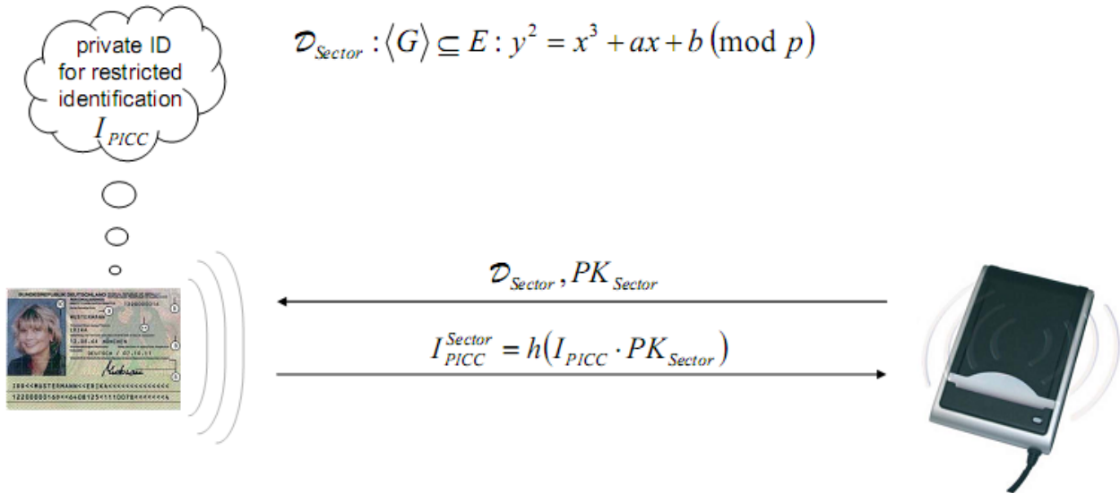
Abbildung 48: Restricted Identification [BSI-TR-03112-7]
