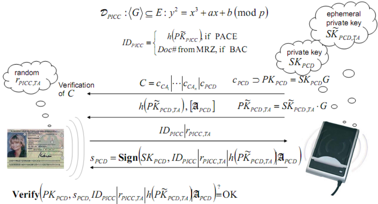
Abbildung 46: Terminal Authentication, Version 2 [BSI-TR-03112-7]
